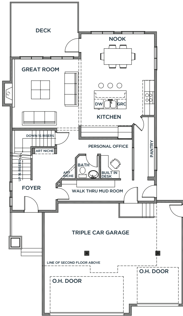
MAIN FLOOR PLAN 1148 SQ.FT
